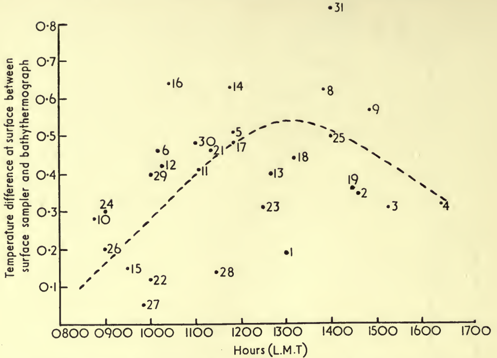
FIG. 3. Difference of temperature between surface samples and bathythermograph 'surface' recordings, plotted against time of day. (Numbers refer to stations.)
